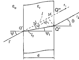
Fig. 6. Ray tracing through a dielectric plate.
