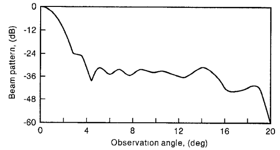
Fig. 8. Beam pattern of quarter-wave Fresnel-zone plate antenna.
