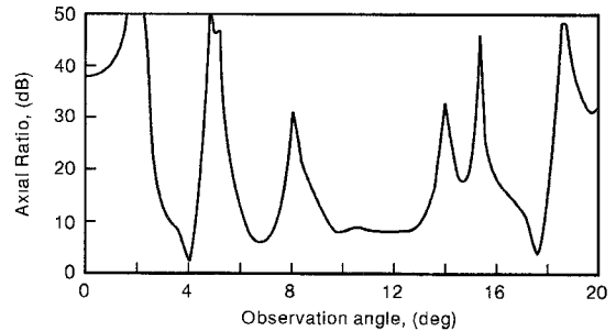
Fig. 9. Axial polarization ratio AR versus observation angle.
